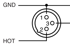
XLR Unbalanced
