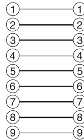
Included RS-232C cable
