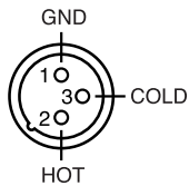
XLR Balanced
